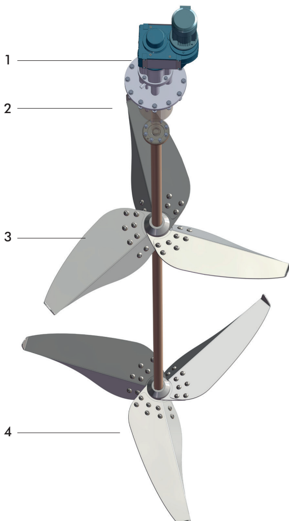
CYBERSLUDGE® Mixer: 3D representation
